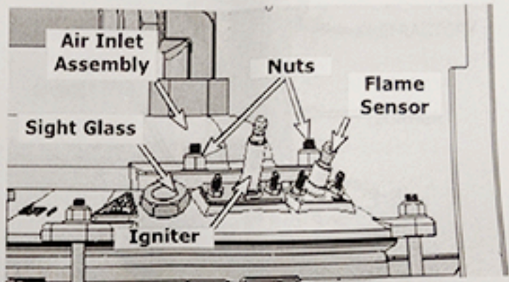
Figure 1 - Sight Glass, Igniter & Flame Sensor
