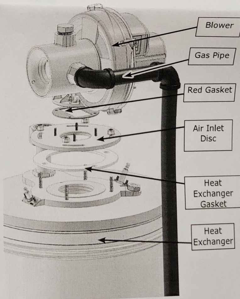
Figure 4 - Blower Assembly
