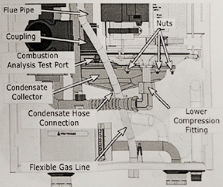
Figure 2 - Condensate Trap
